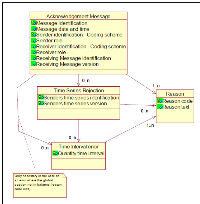
Figure A-2: ESS 2.3 acknowledgement message: Information model
